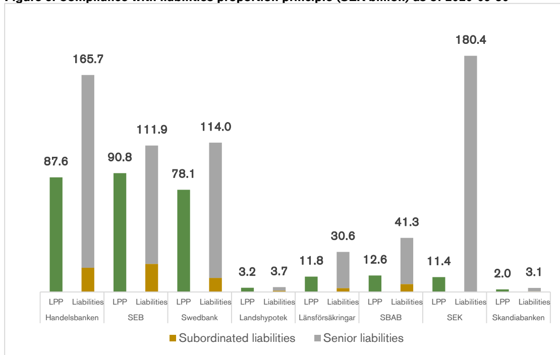
Figure 5. Compliance with liabilities proportion principle (SEK billion) as of 2020-09-30
